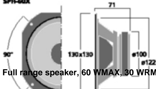
SPH-60X
